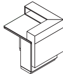
LD03 Right end with transaction box W800 D875 H950/1100 mm
